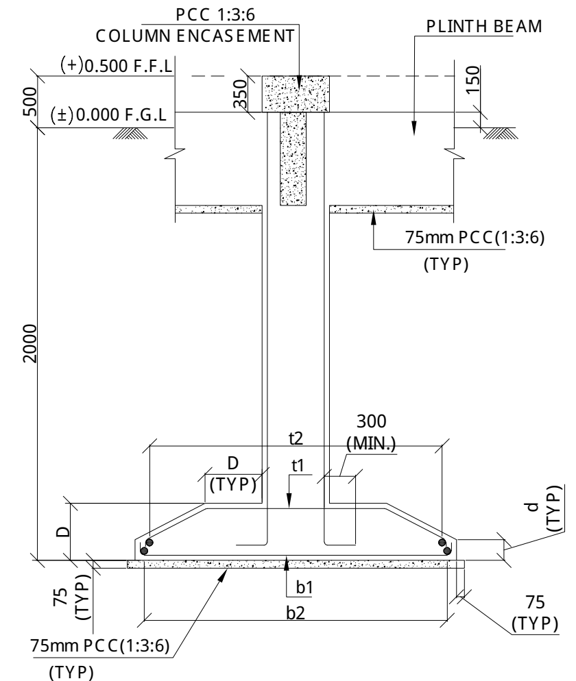
TYP. SECTION A-A OF ISOLATED FOUNDATION
