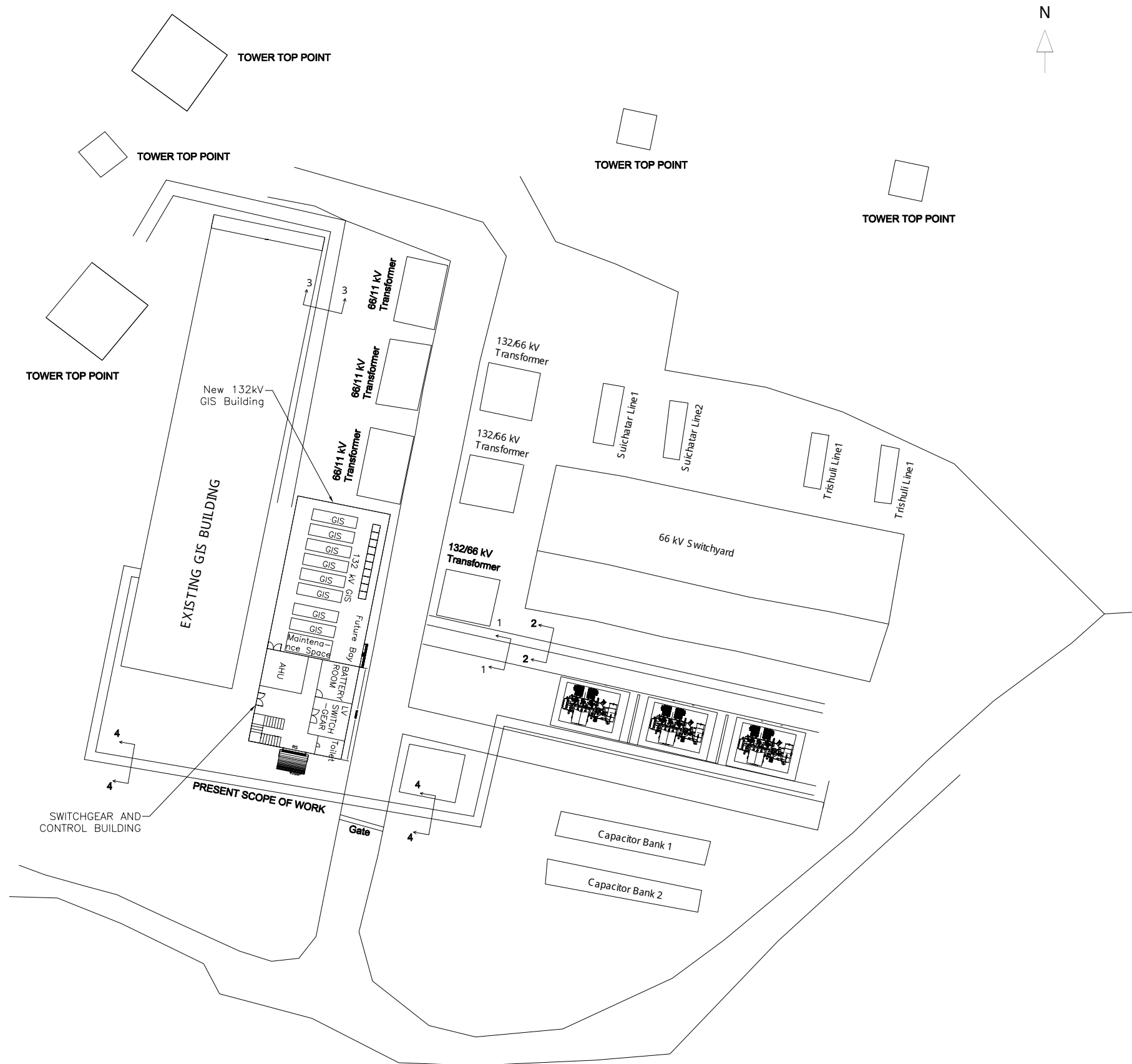
CABLE TRENCH LAYOUT
